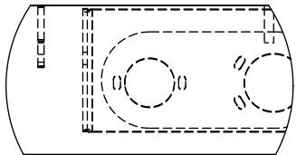
DETAIL B SCALE 1 : 7
